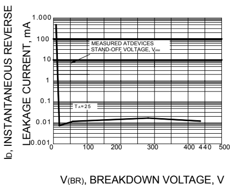
FIG.7 – TYPICAL REVERSE LEAKAGE CHARACTERISTICS
