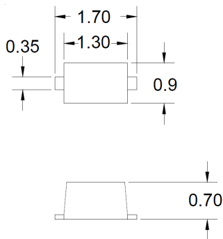
Package Dimensions
